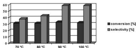
Figure 1. Influence of the temperature on conversion and amine selectivity of the DRA of PhCOMe with BnNH 2 {conditions: 5 mmol PhCOMe, 5 mmol BnNH 2 , 0.01 mmol [Rh(dppb)COD]BF 4 , 10 mL MeOH, 50 bar initial H 2 pressure (measured at RT), exposition time 9 h}.
