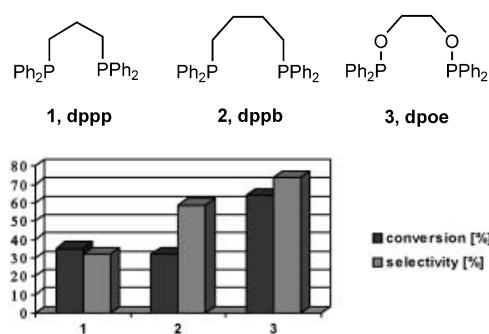
Figure 2. Comparison of the performance of different catalysts in the DRA of PhCOMe with BuNH 2 . 1: [Rh(dppp)COD]BF 4 ; 2: [Rh(dppb)COD]BF 4 ; 3: [Rh(dpoe)COD]BF 4 at 100 °C (for other conditions see Fig. 1).
