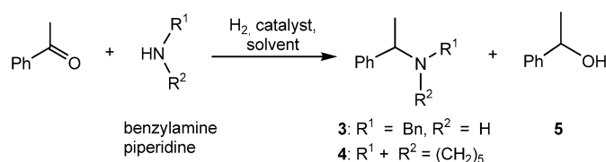
Scheme 2. Reductive amination of acetophenone.
