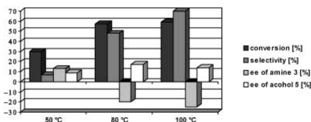
Figure 3. Influence of the temperature on the catalytic performance of [Rh(( R,R )-bdp)COD]BF 4 in the asymmetric DRA of PhCOMe with BuNH 2 (for conditions see Fig. 1). Positive ee values correspond to the ( R )-configuration and negative to the ( S )-configuration.
