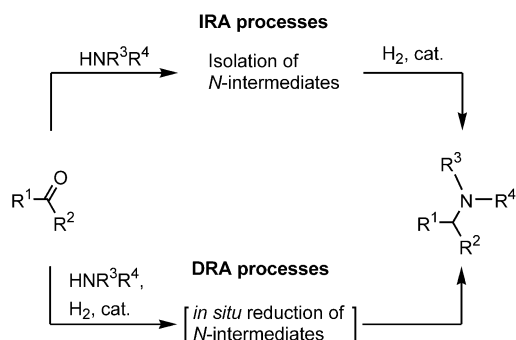
Scheme 1. General approaches for reductive aminations.
